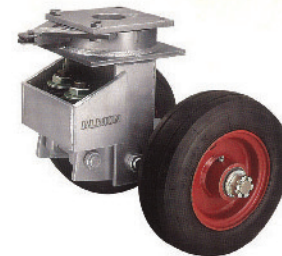
Aviation Ground Equipment (Load Up to 20,000 lbs)
