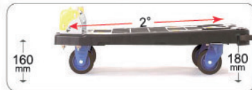
Platform elevated at an angle of 2 degrees
