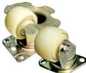
Air Cargo & Conveyor (Diamond Shape Plate/ Toe Guard)
