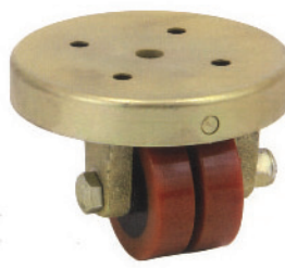
Low Profile 50mm Heavy Duty 160 ~ 270 kg
